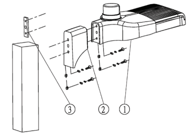
Square Pole Straight Arm
