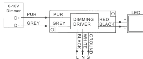
4 WIRING DIAGRAM
