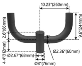
Description: Double Bullhorn with 180° Arms Order Code: BH2V180BZ Color: Bronze Weight: 12 lbs.
