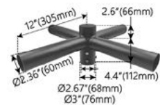
Description: Quad Spoke Accessory with 90° Arms Order Code: SP4H906BZ Color: Bronze Weight: 14 lbs.
