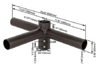
Description: Triple Spoke Accessory with 90° Arms Order Code: SP3H906BZ Color: Bronze Weight: 11.22 lbs.
