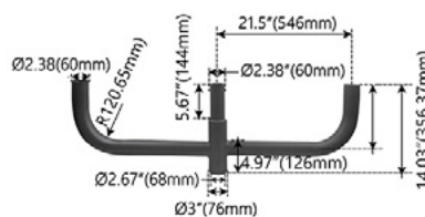
Description: Triple Bullhorn with 180° Arms Order Code: BH3V180BZ Color: Bronze Weight: 18 lbs.
