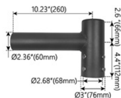
Description: Single Spoke Arm Order Code: SP1H6BZ Color: Bronze Weight: 5 lbs.
